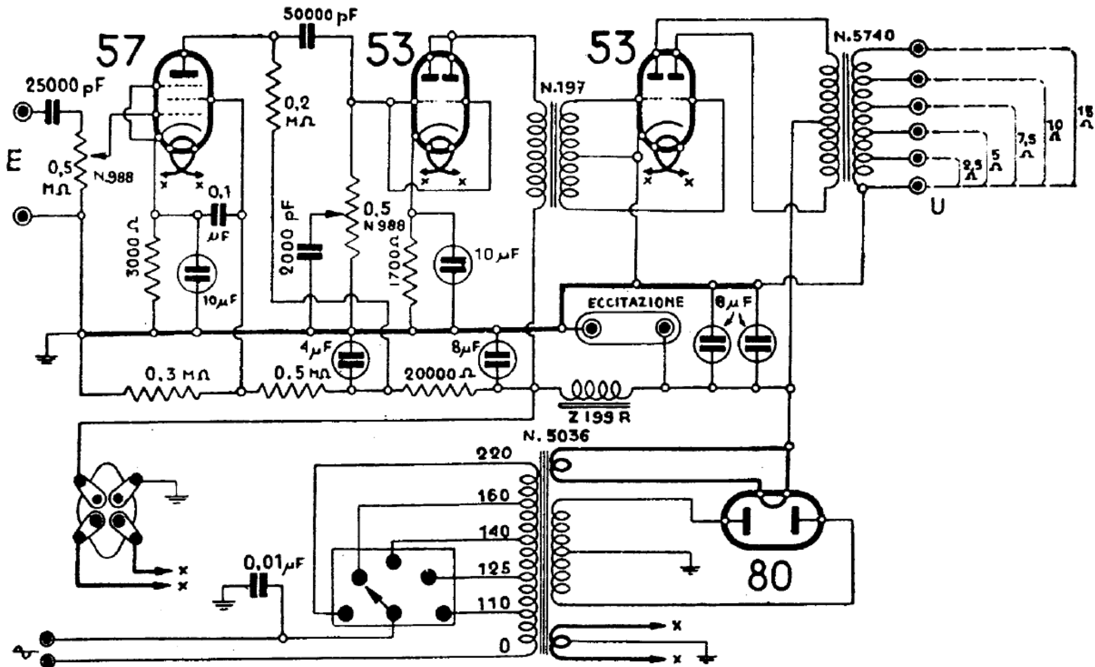
Geloso G17A Amplifier
